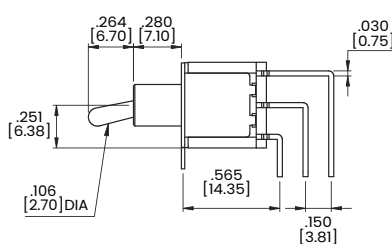
M7 Three Pole
