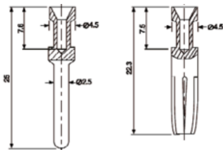
CM-HE Male
