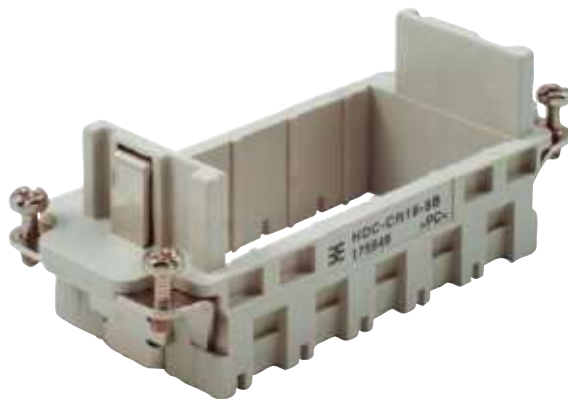
Female frame
