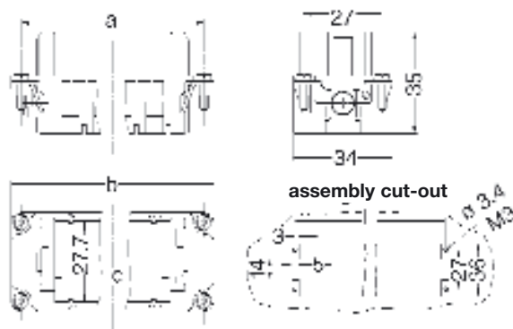
Female frame
