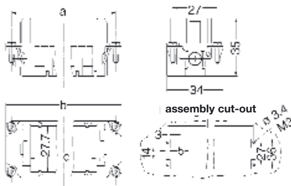
Female frame
