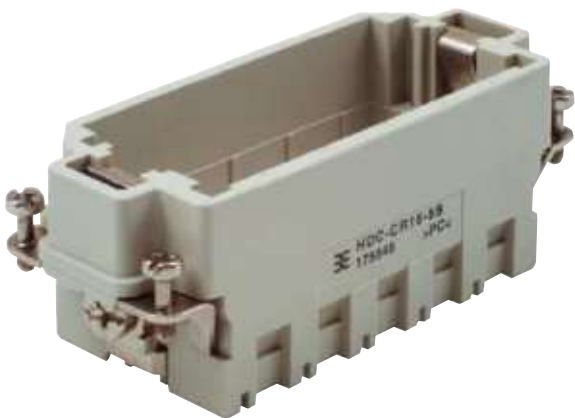
Male frame
