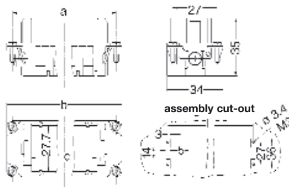
Female frame
