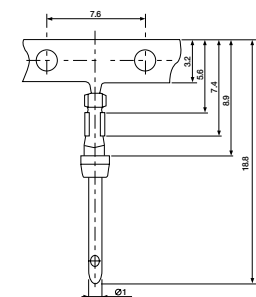
CM-20 Male
