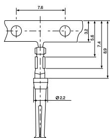
CM-20 Female
