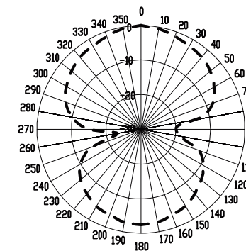
TYPICAL FREE-FIELD POLAR PATTERN AT 125Hz:
