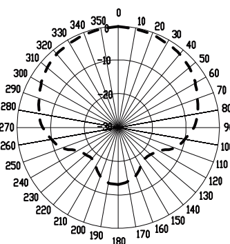
TYPICAL FREE-FIELD POLAR PATTERN AT 1KHz:
