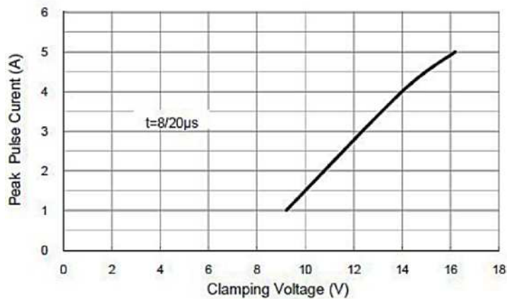
Fig 3 Voltage Sweeping
