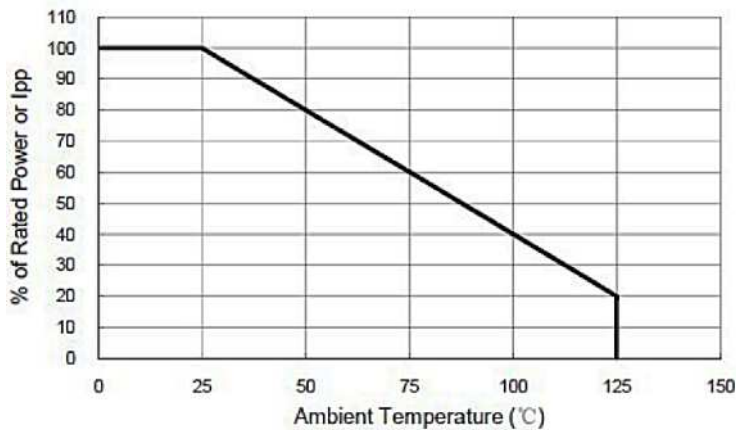
Fig 1 Power Derating Curve
