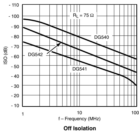
Off Isolation
