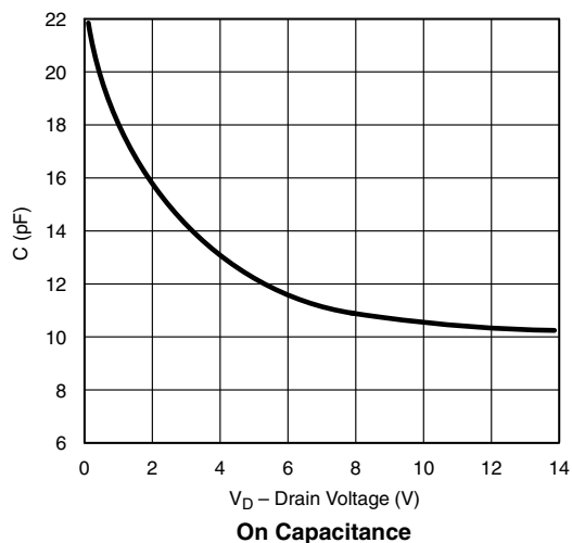
On Capacitance
