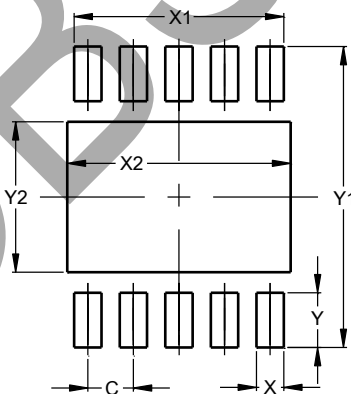
V-DFN3030-10 (Standard)
