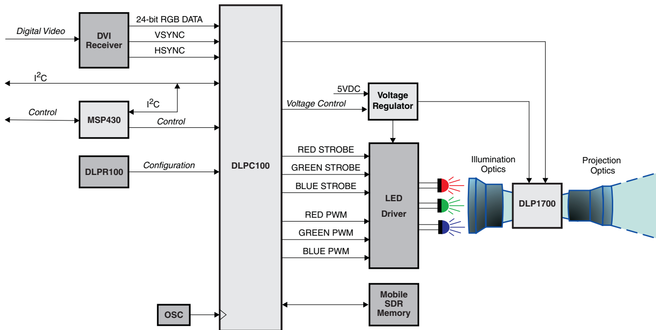
Figure 1. Typical Application
