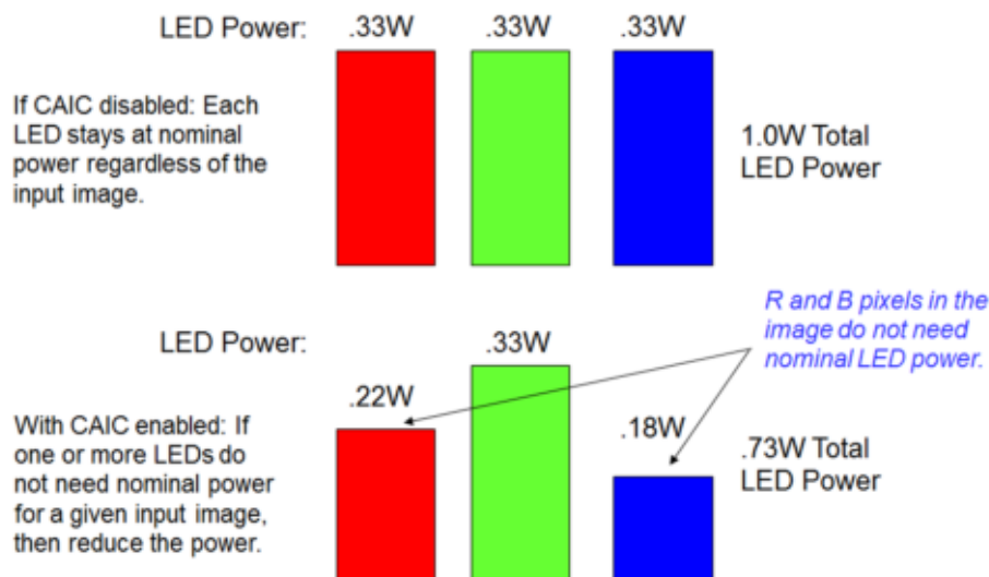
Figure 19. CAIC Power Reduction Mode (for Constant Brightness)
