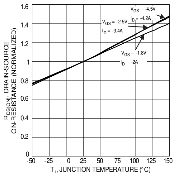
Figure 6 On-Resistance Variation with Junction Temperature
