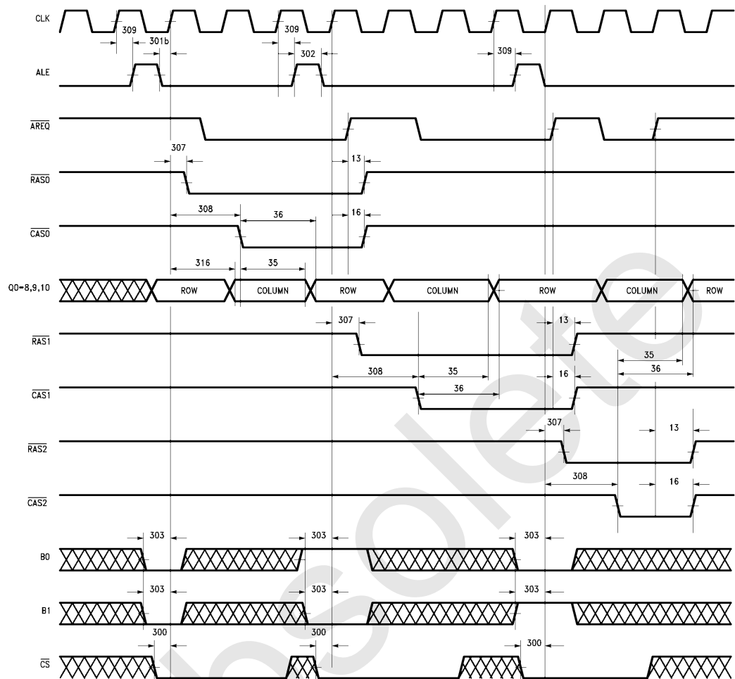
FIGURE 41. 300: Mode 0 Interleaving
