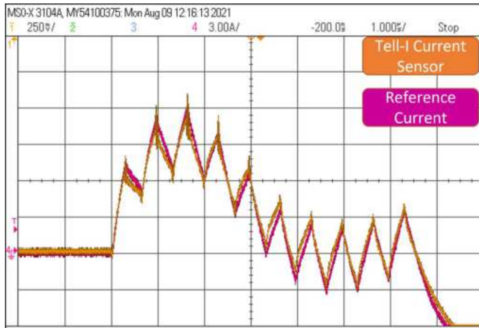
Figure 5. Performance of Tell-i DS10.2m current sensor in a 1.5MHz DC/DC switching converter.
