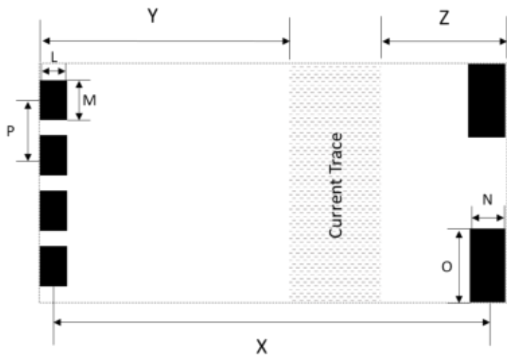
Figure 9 – Recommended Oven/Reflow Soldering PCB Footprint. The recommended Current Trace underneath – NO CONTACT- the sensor is 0.14” (3.56mm) wide.
