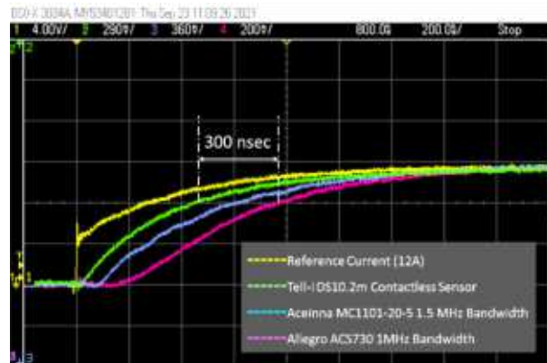
Figure 1. Comparison of DS10.2m vs other sensors
