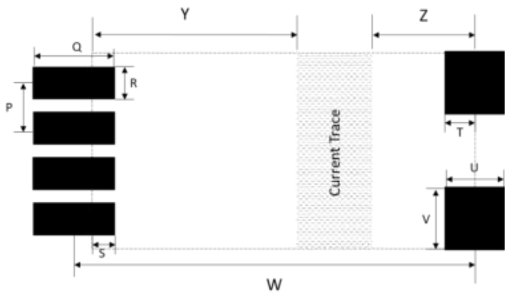
Figure 8 – Recommended Hand Soldering PCB Footprint. The recommended Current Trace underneath – NO CONTACT- the sensor is 0.14” (3.56mm) wide.
