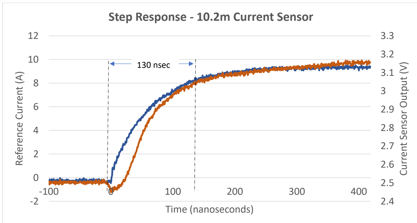
Figure 2. Step Response with 130 nanoseconds risetime.
