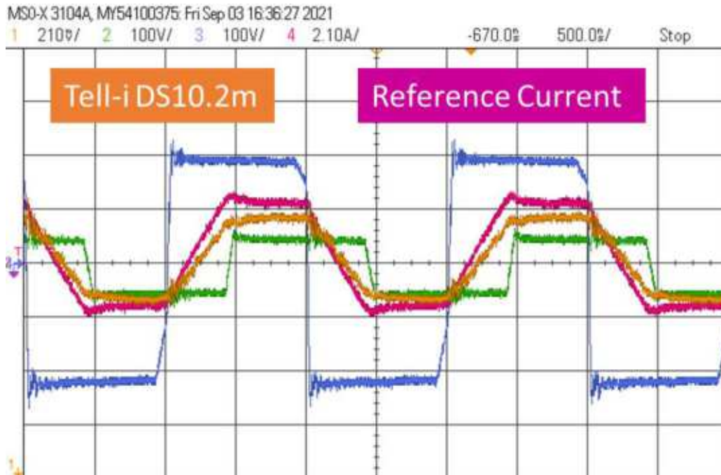
Figure 6. Performance of Tell-i DS10.2m current sensor in a 500kHz isolated Dual Active Bridge (DAB) DC/DC power converter.
