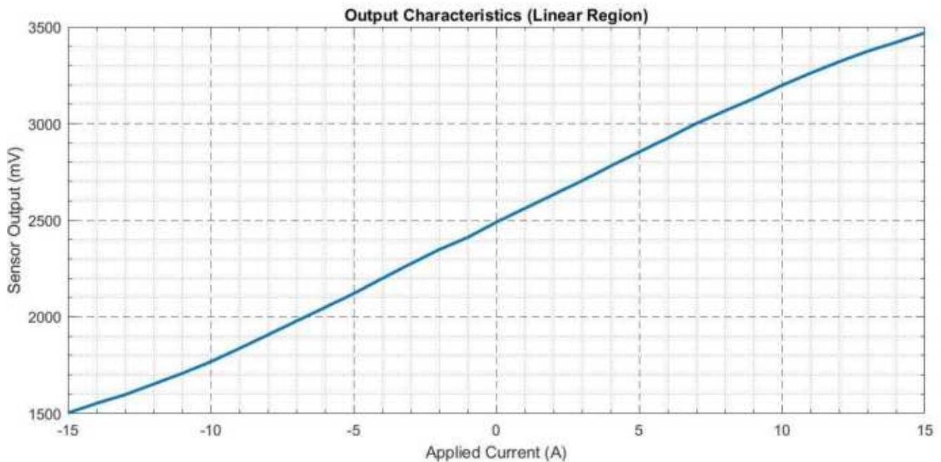
Figure 4. Output Characteristics of the sensor DS10.2m
