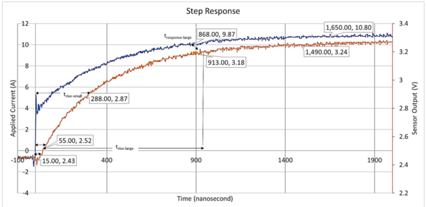
Figure 3. – DS10.2m step response with 868 microsecond rise time – voltage measurement including the line inductance.
