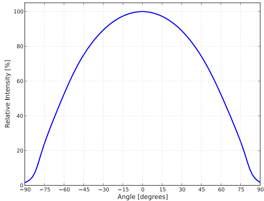
Figure 2: Typical radiation pattern for LUXEON M at 700mA, T j =85°C.
