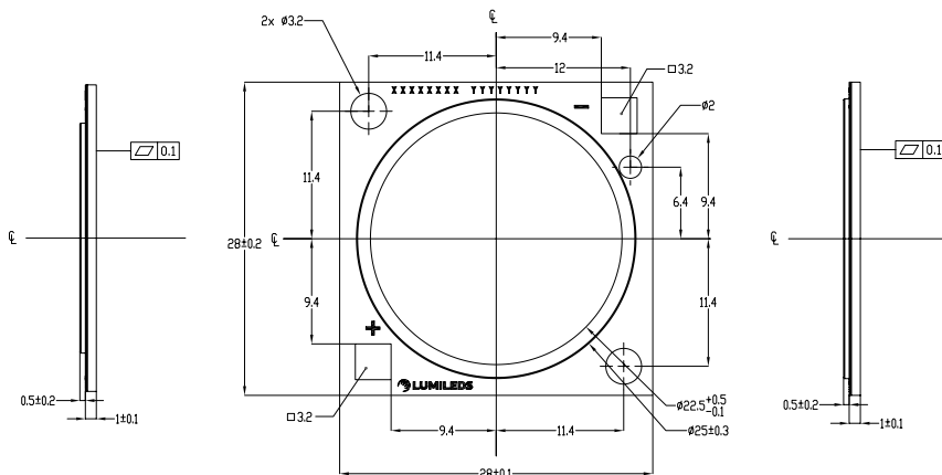
L2C5-xxxx1213x2300, L2C5-xxxx1216x2300 and L2C5-xxxx1812x2300
