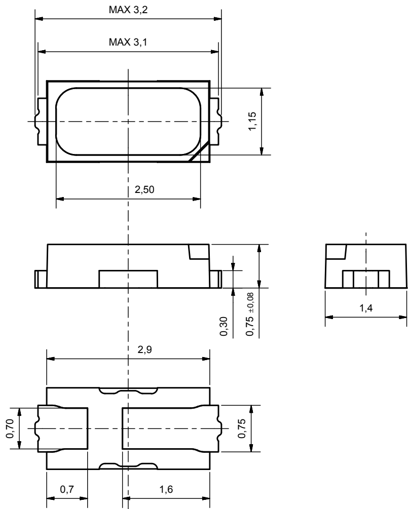
Figure 9. Mechanical dimensions for LUXEON 3014 with FreshFocus Technology.
