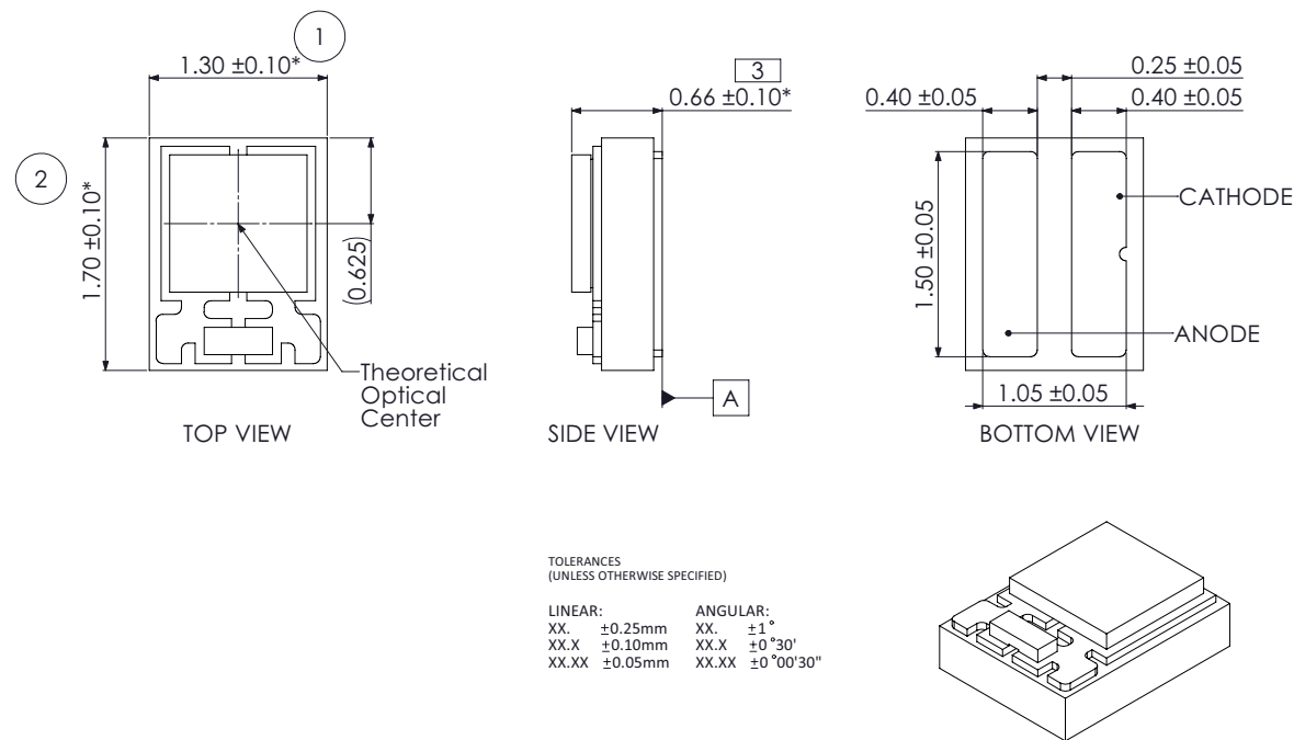
Figure 10a. Mechanical dimensions for LUXEON UV U1.
