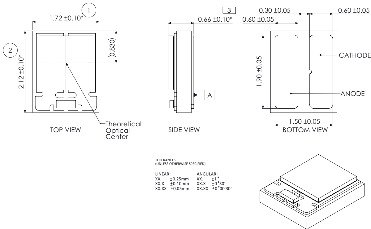
Figure 10b. Mechanical dimensions for LUXEON UV U2.
