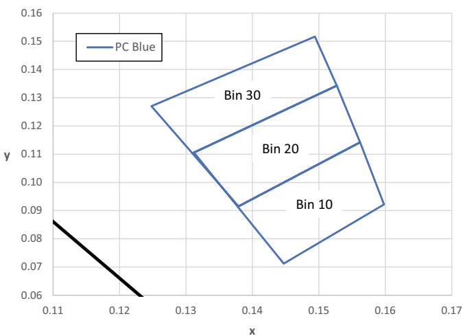
Figure 9. Color bin structure for LUXEON C PC Blue for Table 7.
