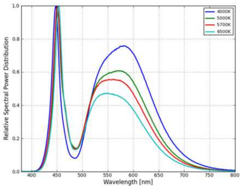
Figure 1a. Typical normalized power vs. wavelength for LUXEON 3535L 70CRI White at 100mA, Tj=25°C.
