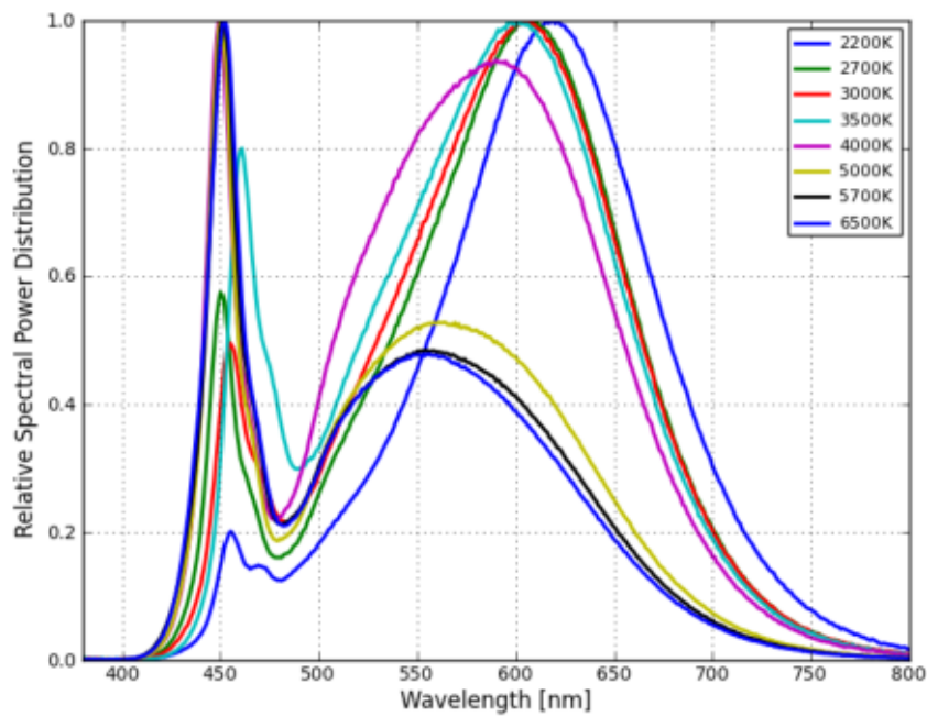
Figure 1b. Typical normalized power vs. wavelength for LUXEON 3535L 80CRI White at 100mA, Tj=25°C.
