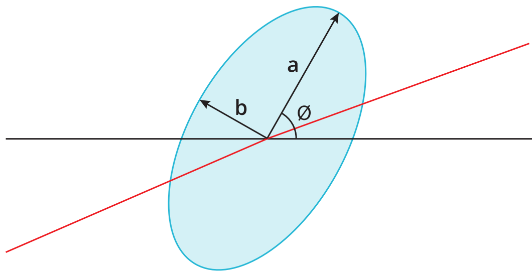
Figure 7. 3-, 4- and 5-step MacAdam ellipse illustration for Tables 6a–6k
