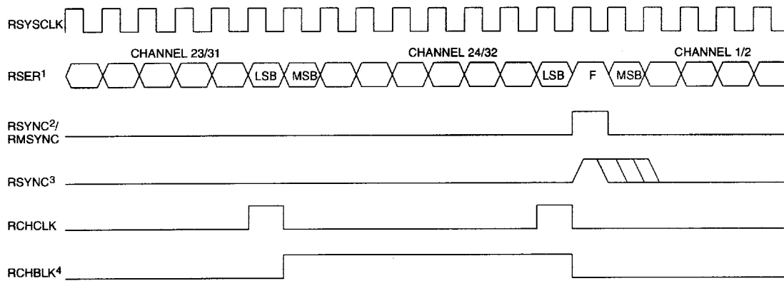
Figure 14-3. Receive Side 1.544MHz Boundary Timing (with Elastic Store Enabled)
