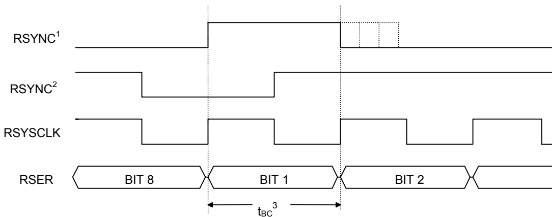
Figure 8-6. RSYNC Input in H.100 (CT Bus) Mode
