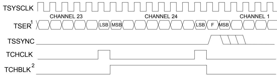
Figure 10-21. E1 Transmit-Side 1.544MHz Boundary Timing (Elastic Store Enabled)
