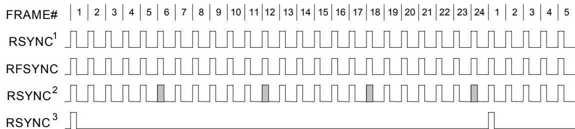
Figure 10-2. T1 Receive-Side ESF Timing
