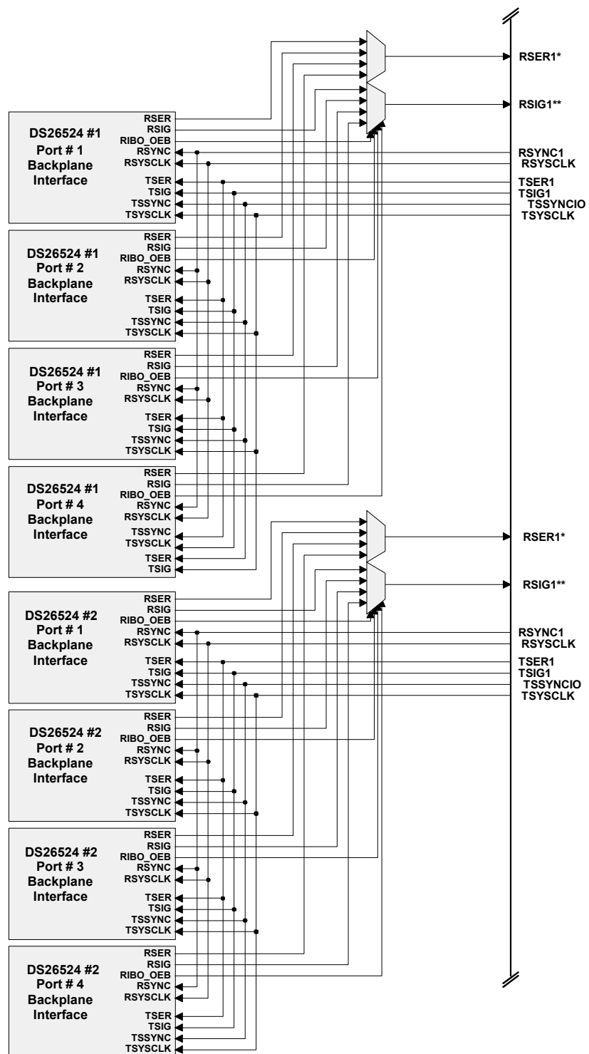
Figure 8-5. IBO Multiplexer Equivalent Circuit—16.384MHz
