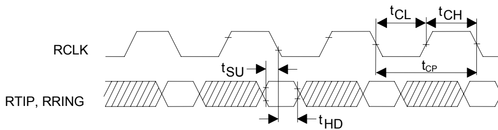
Figure 12-7. Receive Framing Timing—Line Side
