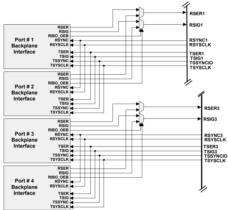
Figure 8-3. IBO Multiplexer Equivalent Circuit—4.096MHz
