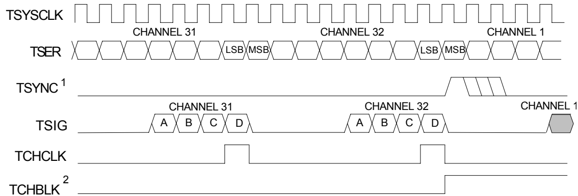
Figure 10-22. E1 Transmit-Side 2.048MHz Boundary Timing (Elastic Store Enabled)
