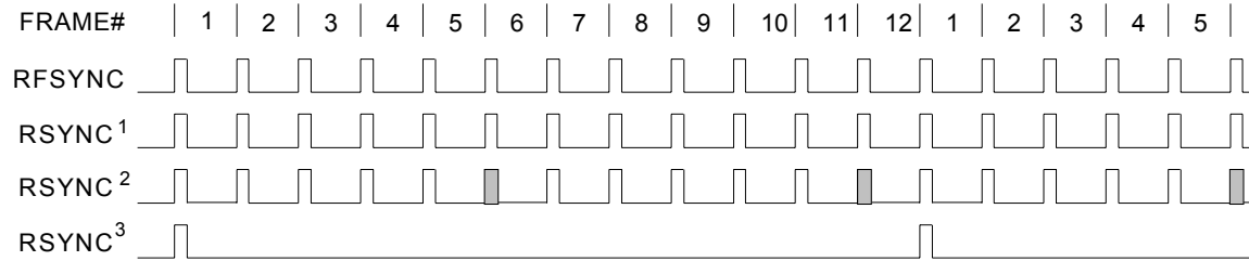
Figure 10-1. T1 Receive-Side D4 Timing
