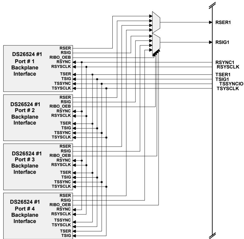
Figure 8-4. IBO Multiplexer Equivalent Circuit—8.192MHz
