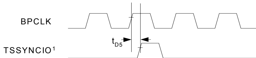
Figure 12-10. BPCLK Timing
