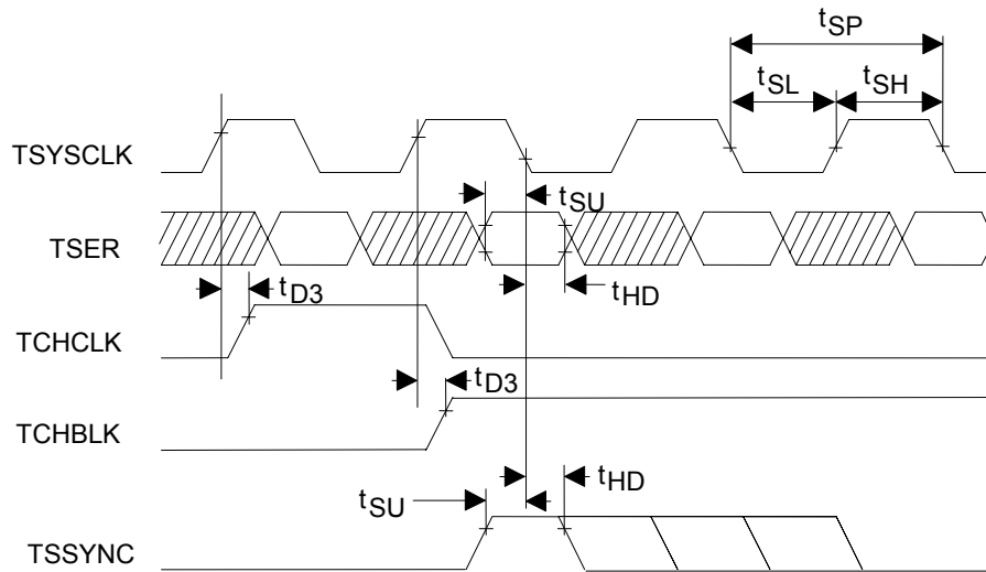
Figure 12-9. Transmit Formatter Timing, Elastic Store Enabled
