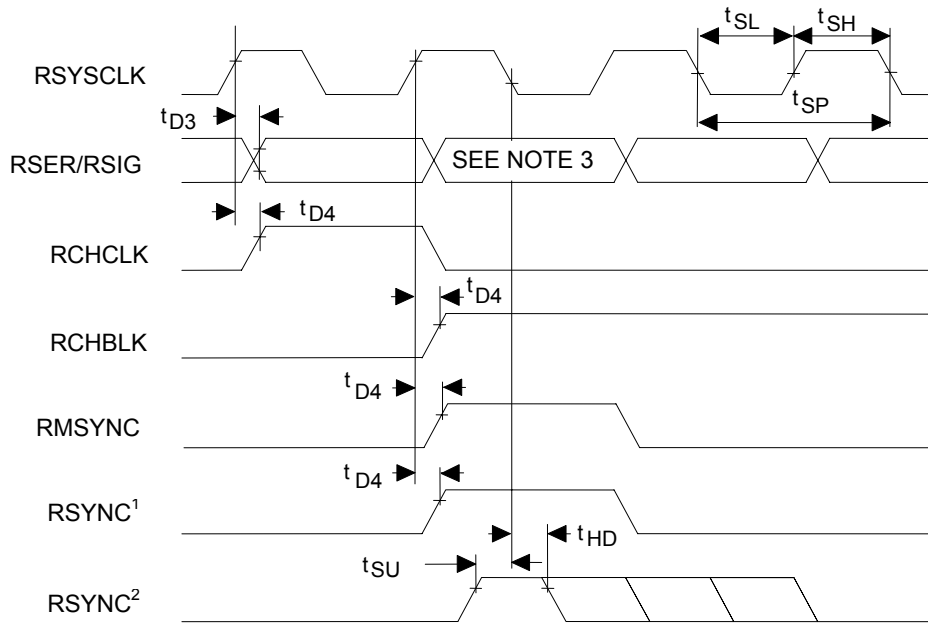
Figure 12-6. Receive-Side Timing, Elastic Store Enabled (T1 Mode)
