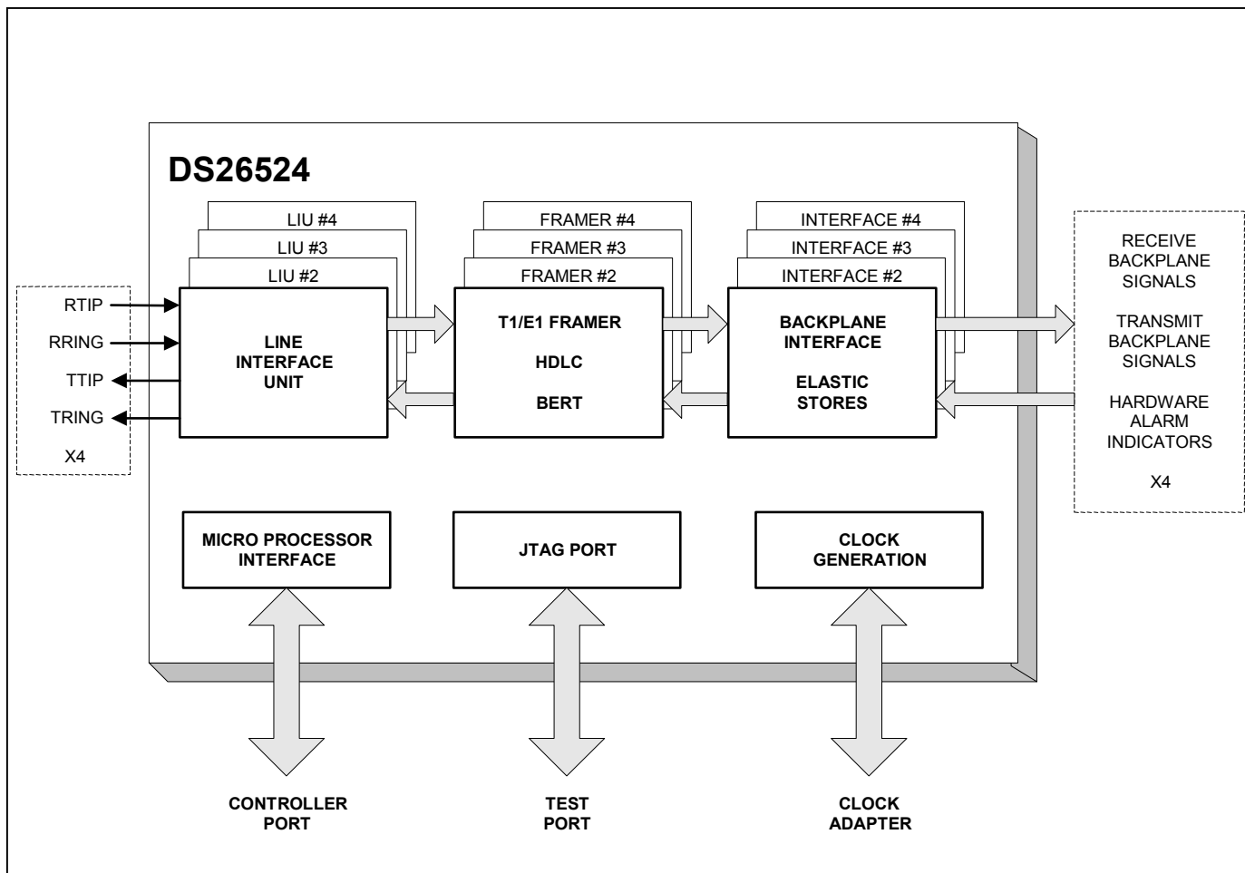
Figure 6-1. Block Diagram
