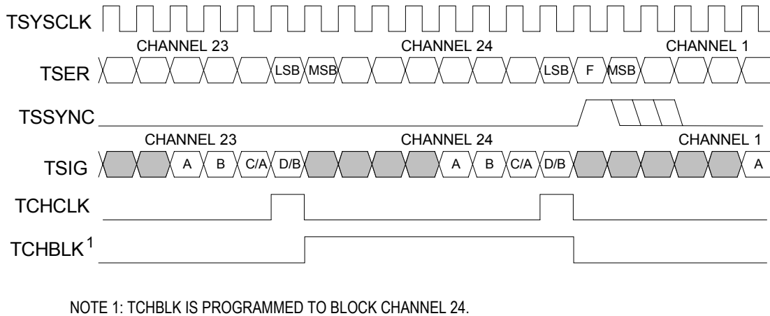
Figure 10-11. T1 Transmit-Side 1.544MHz Boundary Timing (Elastic Store Enabled)
