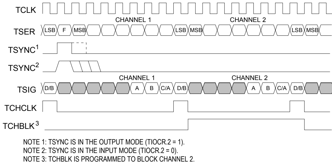
Figure 10-10. T1 Transmit-Side Boundary Timing (Elastic Store Disabled)
