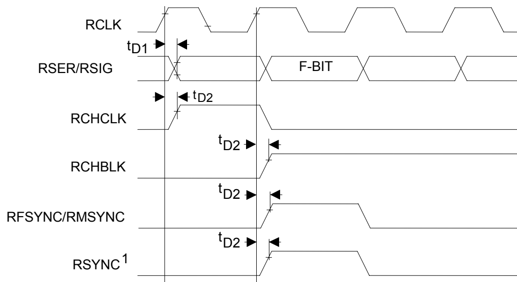
Figure 12-5. Receive Framer Timing—Backplane (T1 Mode)
