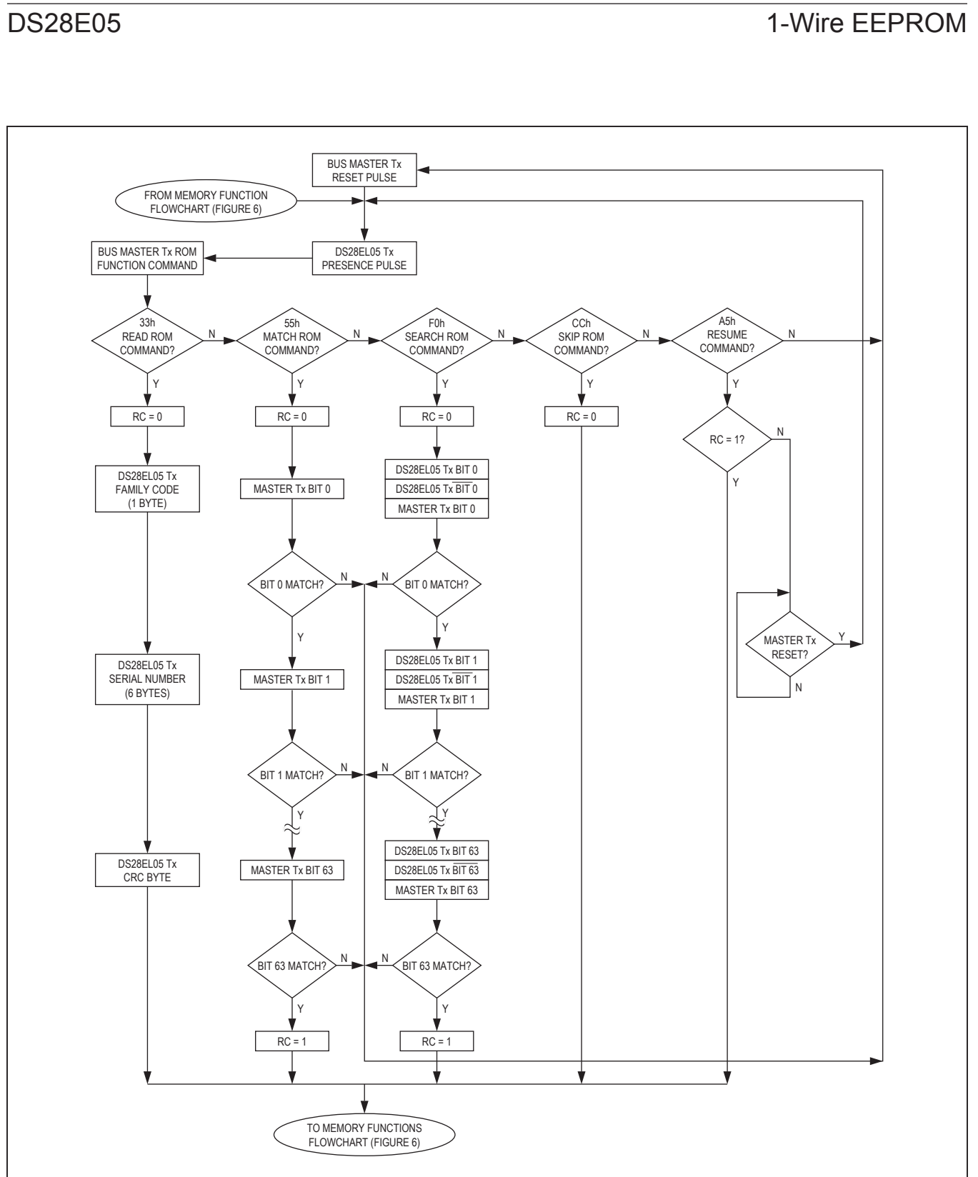
Figure 8. ROM Functions Flowchart
