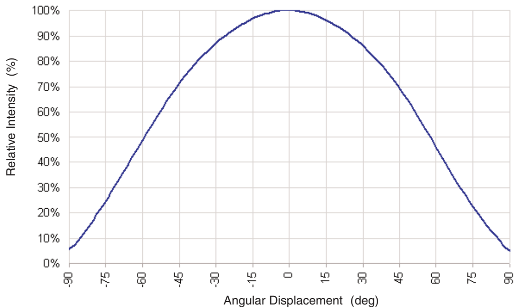
Figure I Ia. Typical representative spatial radiation pattern for cool-white and neutral-white lambertian.
