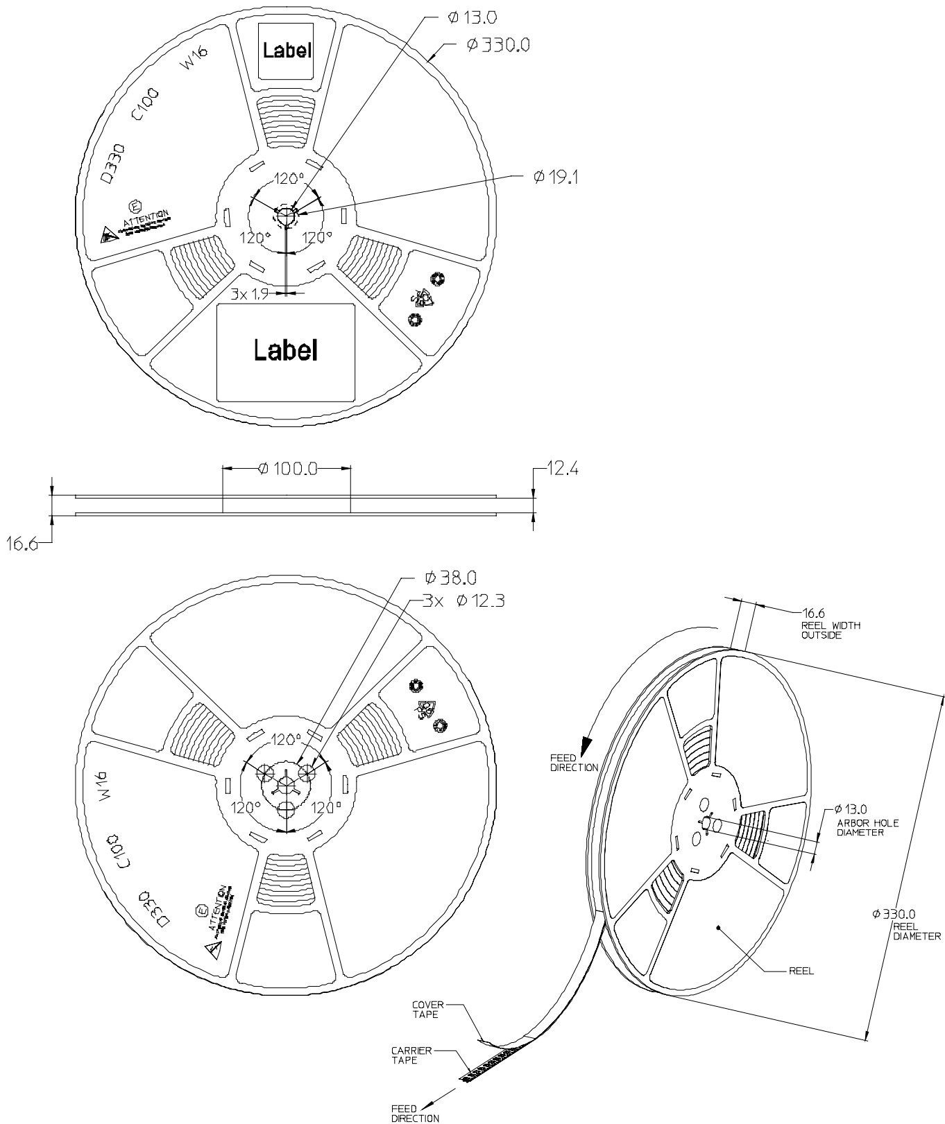
Figure 14. Emitter reel packageing
