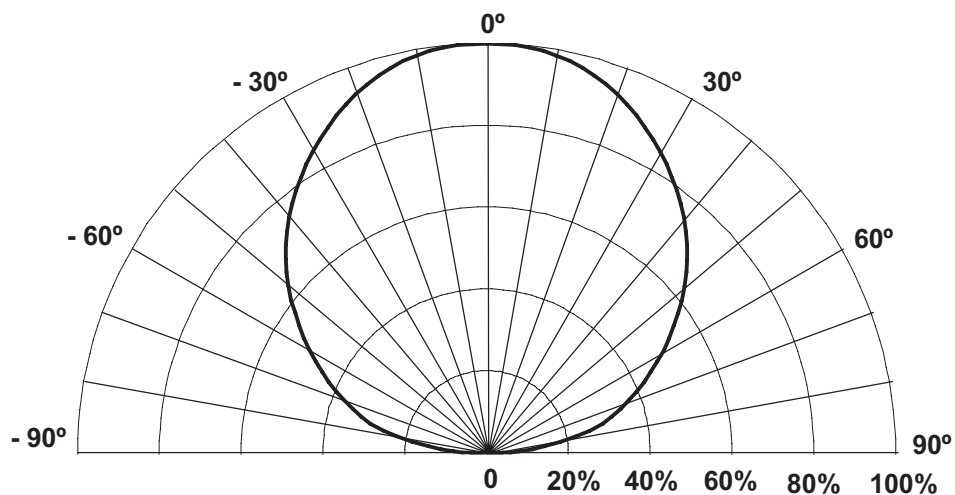
Figure I Ib. Typical polar radiation pattern for cool-white and neutral-white lambertian.
