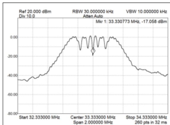
FIGURE 3-2: DSA612 Spectrum at 33.333 MHz with Modulation Turned On.
