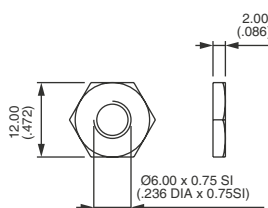
SPECIAL NUT 12 (.472) ACROSS FLATS
