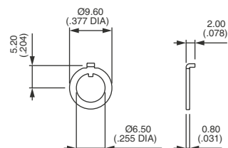
LOCKING RING
