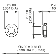
KNURLED CAP NUTS
