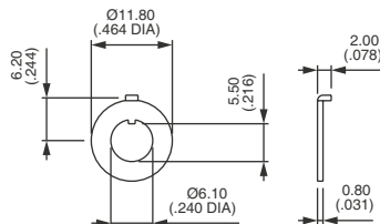
LOCKING RING
