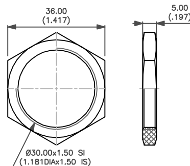
HEX NUT FOR MODELS Ø 30 (1.181)
