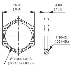
HEX NUT FOR MODELS Ø 22 (.866)
