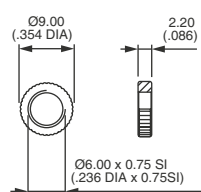
KNURLED NUT
