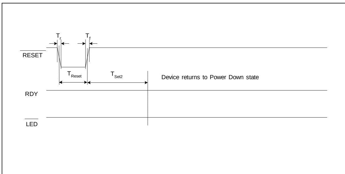
Figure 12.6: Reset Operation
