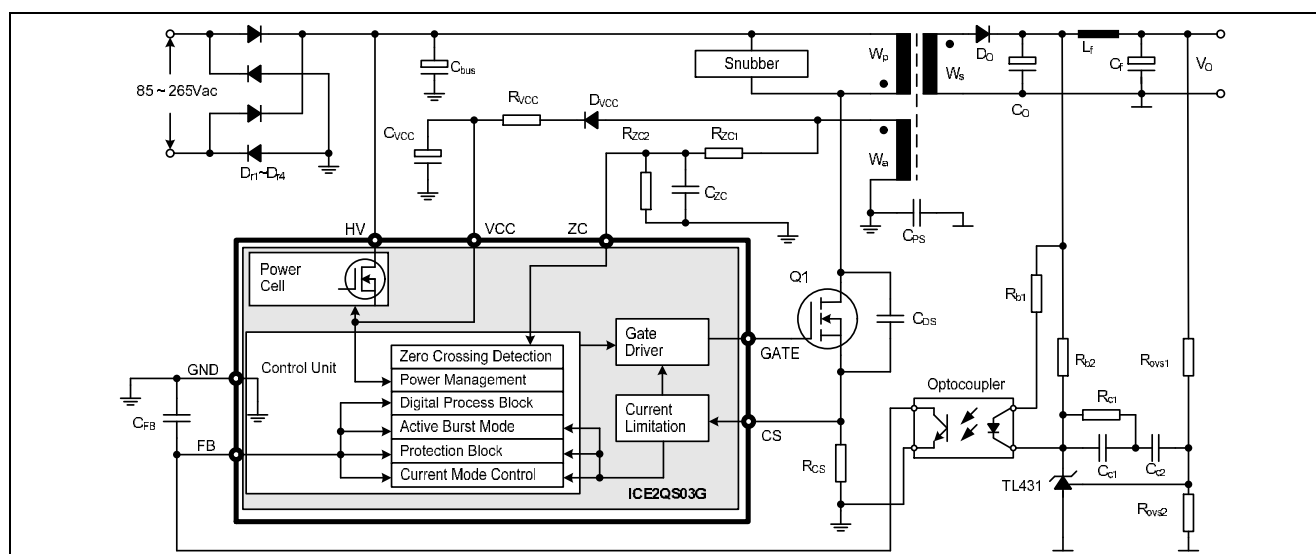
Figure 1 Typical Application
