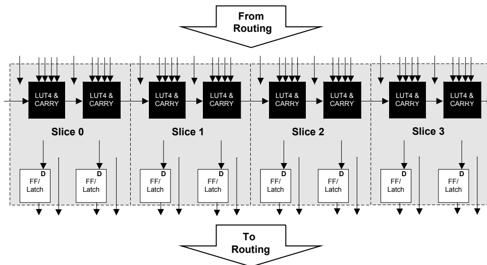
Figure 2-3. PFU Diagram
