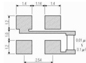
Figure 2) Land Pattern
