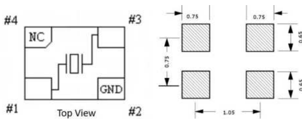
Figure 2) Suggested land pattern
