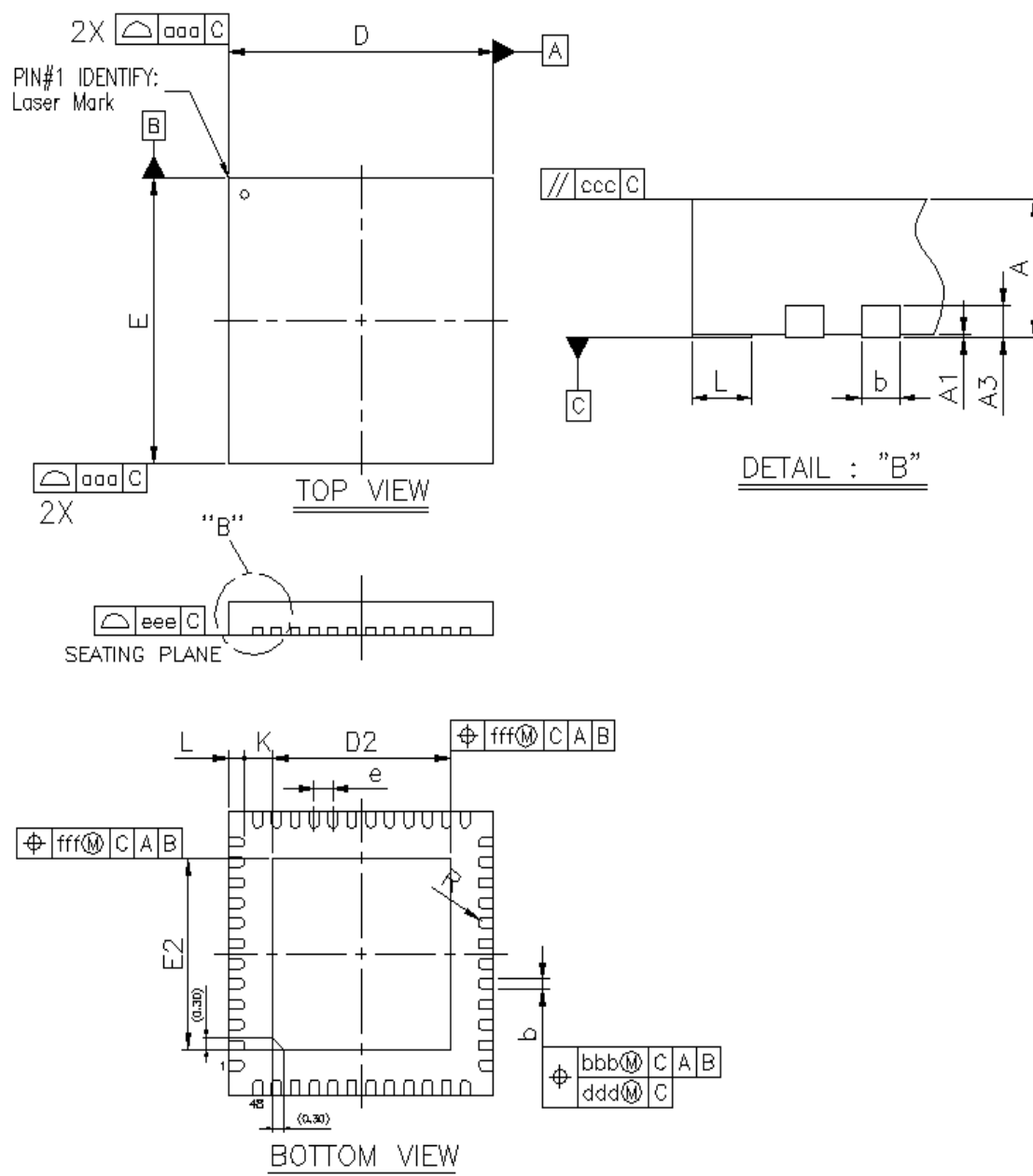
Figure 6.3. QFN48 Package Drawing
