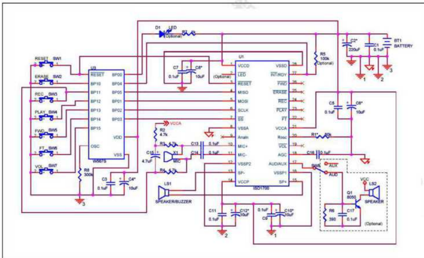
Example #4: Connecting the ISD1700 with PowerSpeech W567
