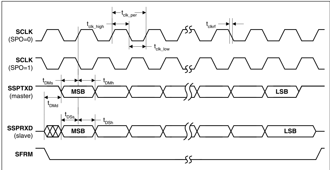
Figure 20. SPI Format with SPH=1 Timing Measurement
