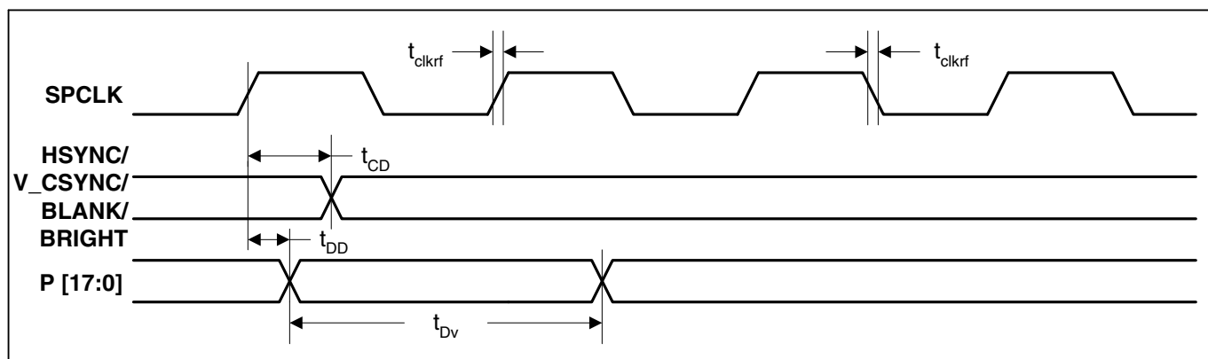
Figure 23. LCD Timing Measurement
