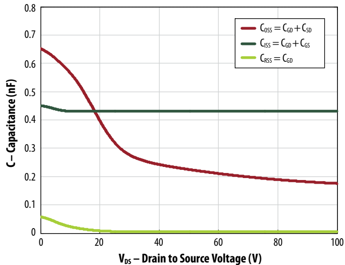
Figure 5: Capacitance
