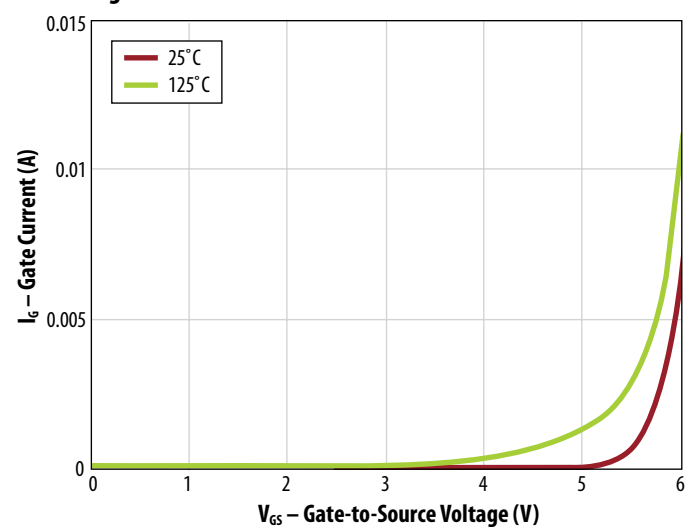
Figure 10: Gate Current
