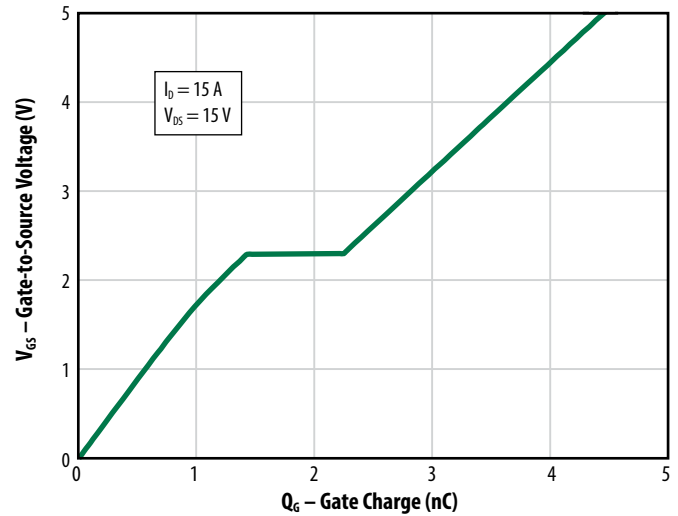
Figure 7b (Q2): Typical Gate Charge
