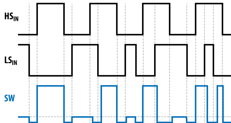
Figure 5: Input-to-Output Timing Diagram (Current flowing OUT of SW node)
