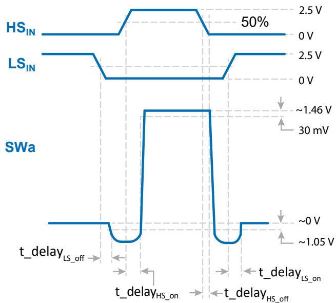
Figure 4b: Logic Input to Switch-node Waveforms
