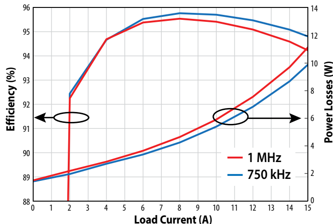
Figure 1: Performance Curves
