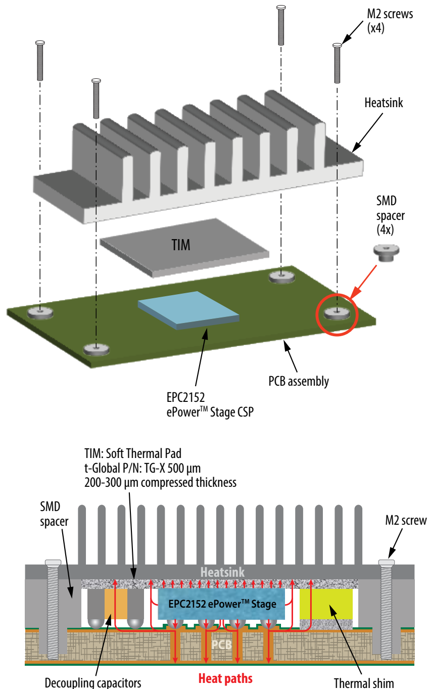
Figure 8: Thermal Concept of Dual Sided Cooling
