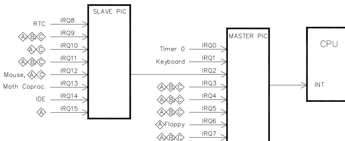
Figure 8. Interrupt Circuit Diagram
