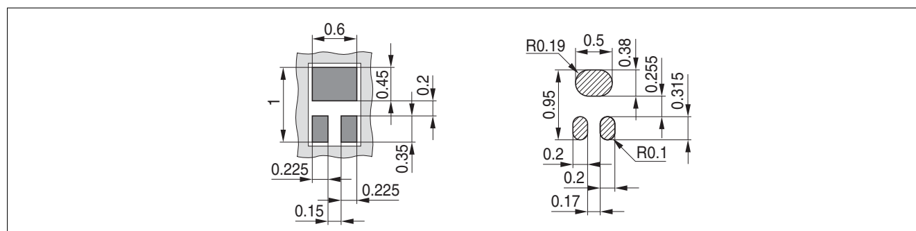
Figure 4-2 TSLP-3-9 Footprint
