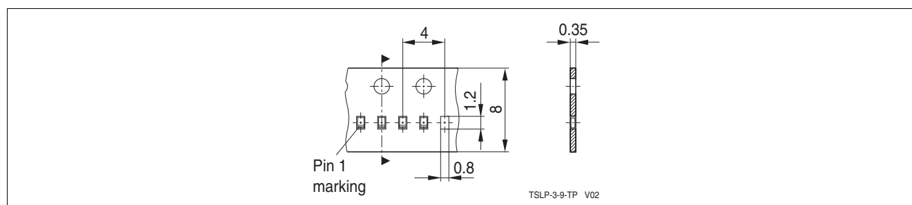
Figure 4-3 TSLP-3-9 Packing
