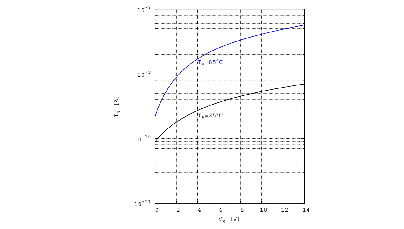
Figure 5 Reverse characteristic, I_R = (V_R) , T_A = \text{parameter}
