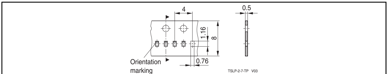
Figure 17 PG-TSLP-2-7: Packing
