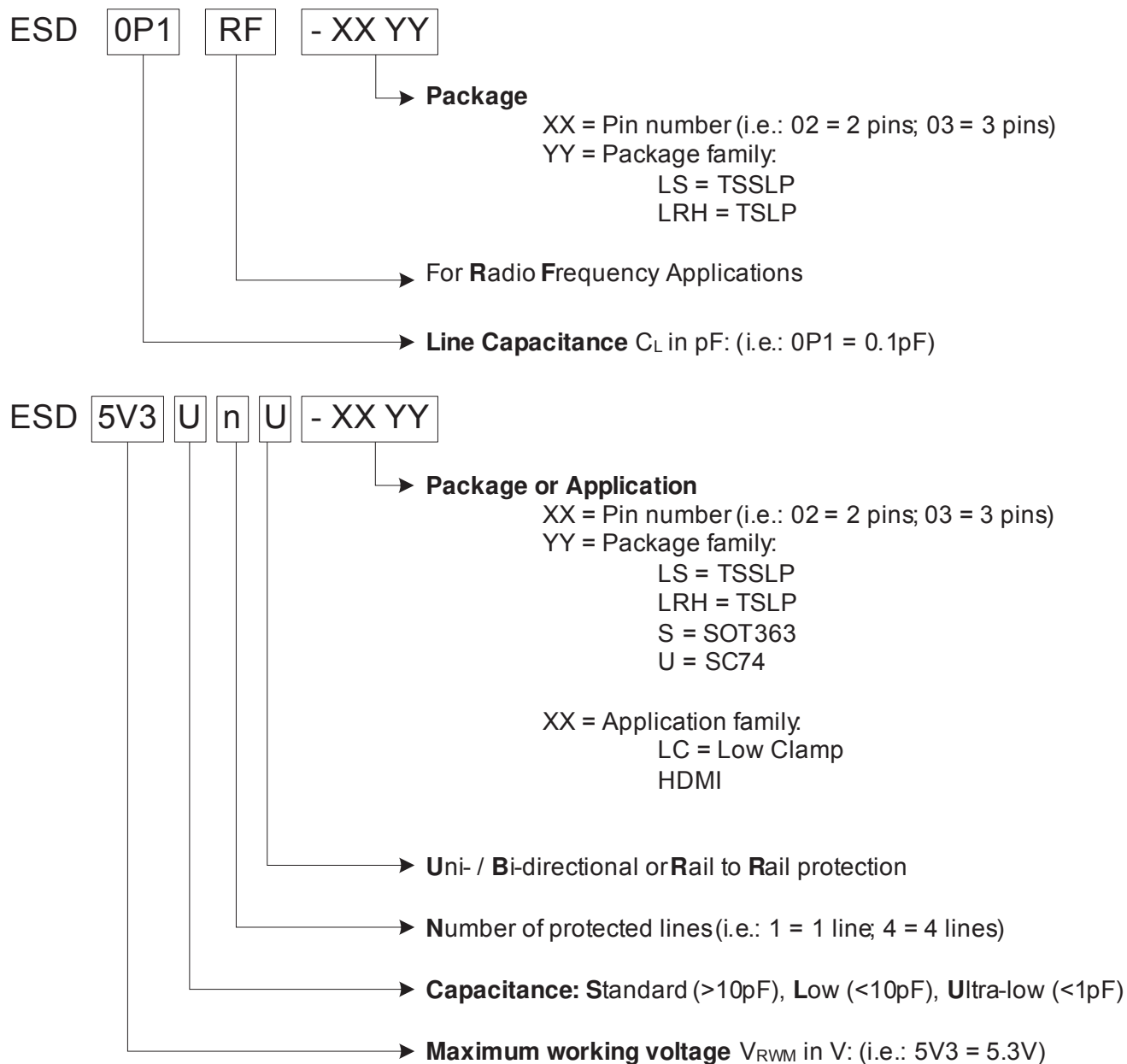
Figure 8 Ordering Information Scheme (examples)
