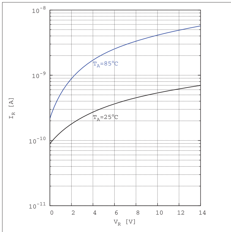
Figure 5 Reverse characteristic, I_R = (V_R) , T_A = \text{parameter}
