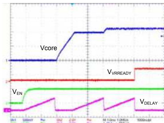
Figure 9: Start-up Waveforms
