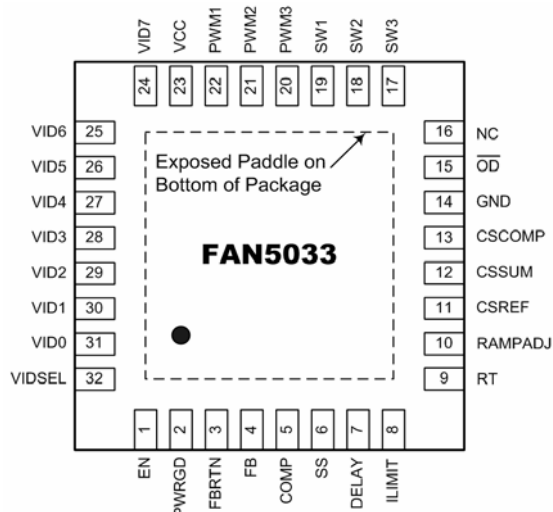
Figure 2: Pin Assignment
