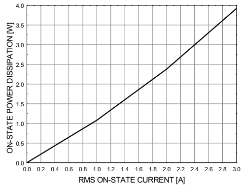
Figure 8. Maximum On-state Power Dissipation
