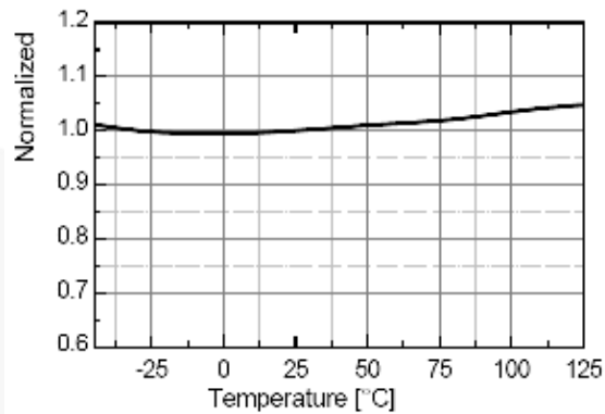
Figure 14. Maximum On-Time Program 1 ( t_{ON,MAX1} ) vs. T_A
