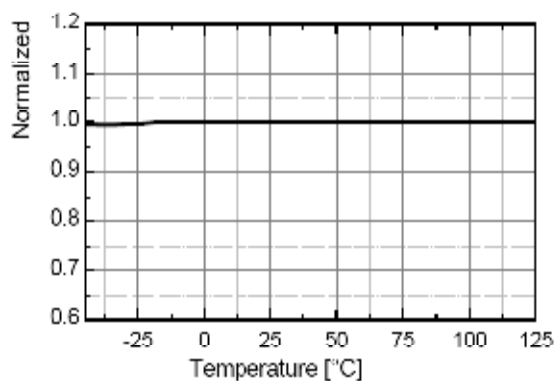
Figure 13. Zero Duty Cycle Output Voltage ( V_{EAZ} ) vs. T_A
