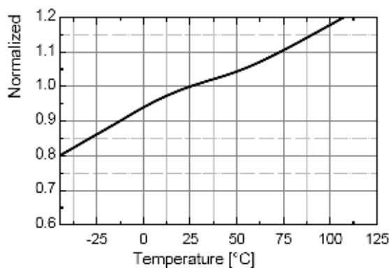
Figure 23. Output Saturation Voltage ( V_{RDY, SAT} ) vs. T_A
