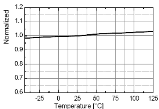
Figure 17. Input High Clamp Voltage ( V_{CLAMPH} ) vs. T_A
