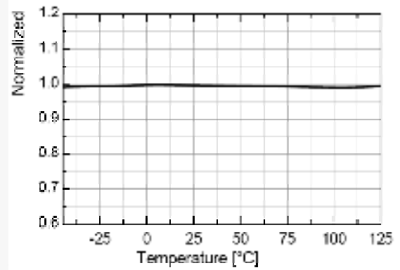
Figure 22. OVP Threshold at OVP Pin ( V_{OVP, OVP} ) vs. T_A
