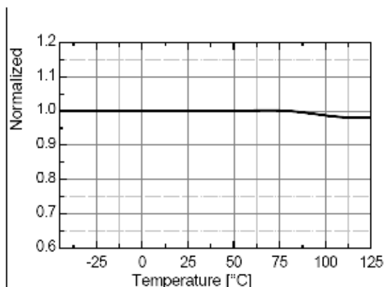
Figure 19. Output Voltage High ( V_{OH} ) vs. T_A
