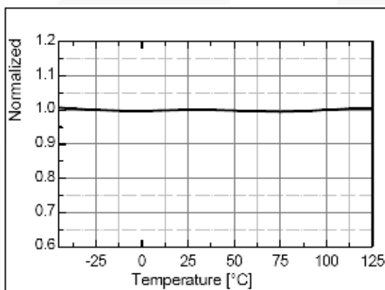
Figure 15. Maximum On-Time Program 2 ( t_{ON,MAX2} ) vs. T_A
