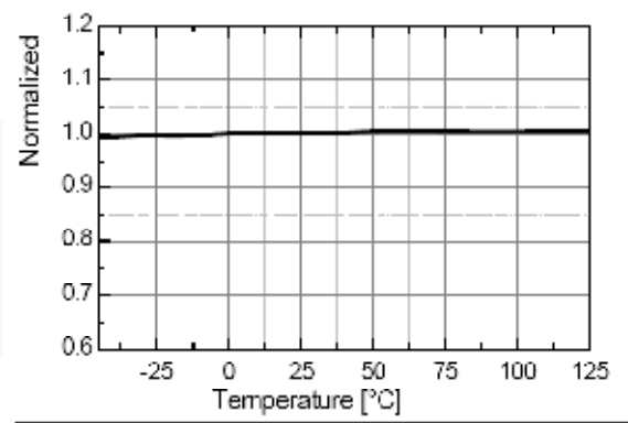
Figure 24. OVP Threshold Voltage ( V_{OVP} ) vs. T_A
