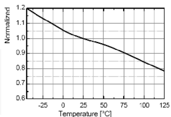
Figure 18. Input Low Clamp Voltage ( V_{CLAMPL} ) vs. T_A
