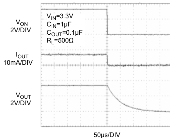
Figure 12. FPF1003 T_{OFF} Response
