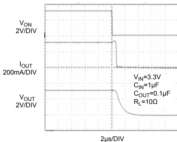
Figure 18. FPF1004 T_{OFF} Response
