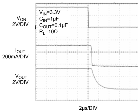
Figure 14. FPF1003 T_{OFF} Response
