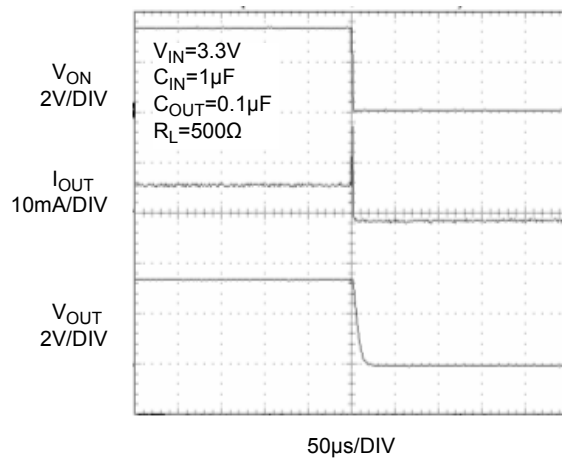
Figure 16. FPF1004 T_{OFF} Response
