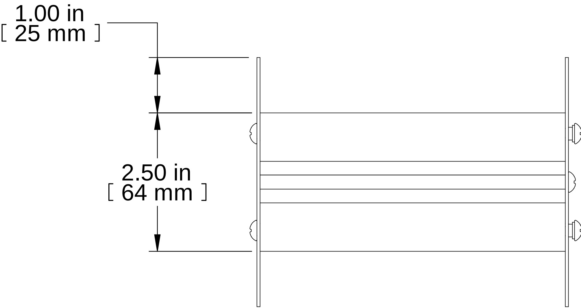
R.S. VIEW
