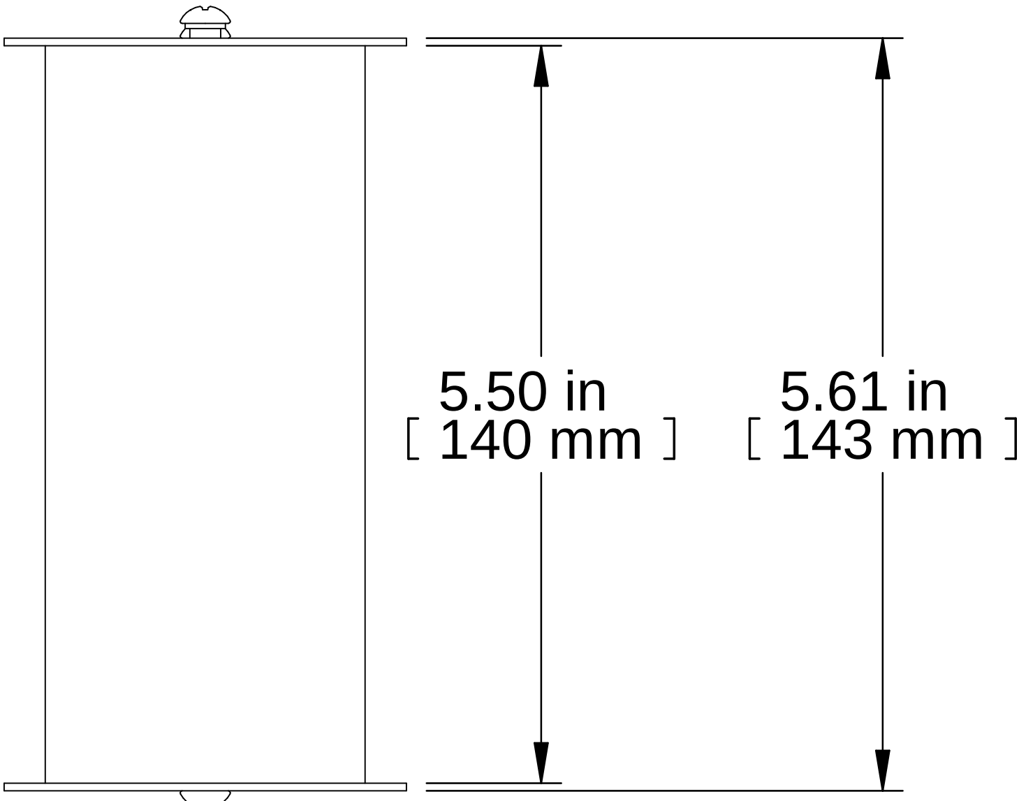
TOP VIEW
