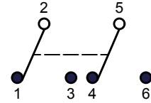
DPDT SCHEMATIC
