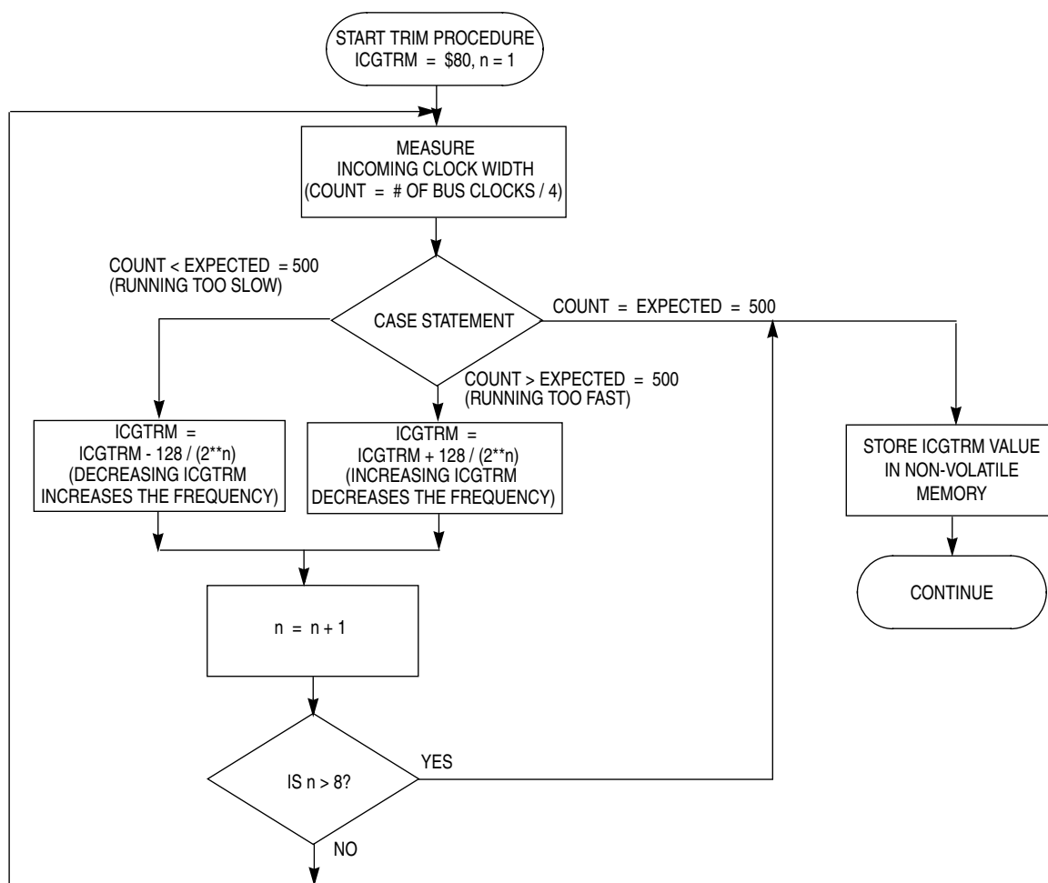
Figure 9-17. Trim Procedure
