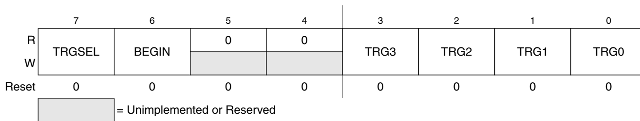
Figure 15-8. Debug Trigger Register (DBGTR)
