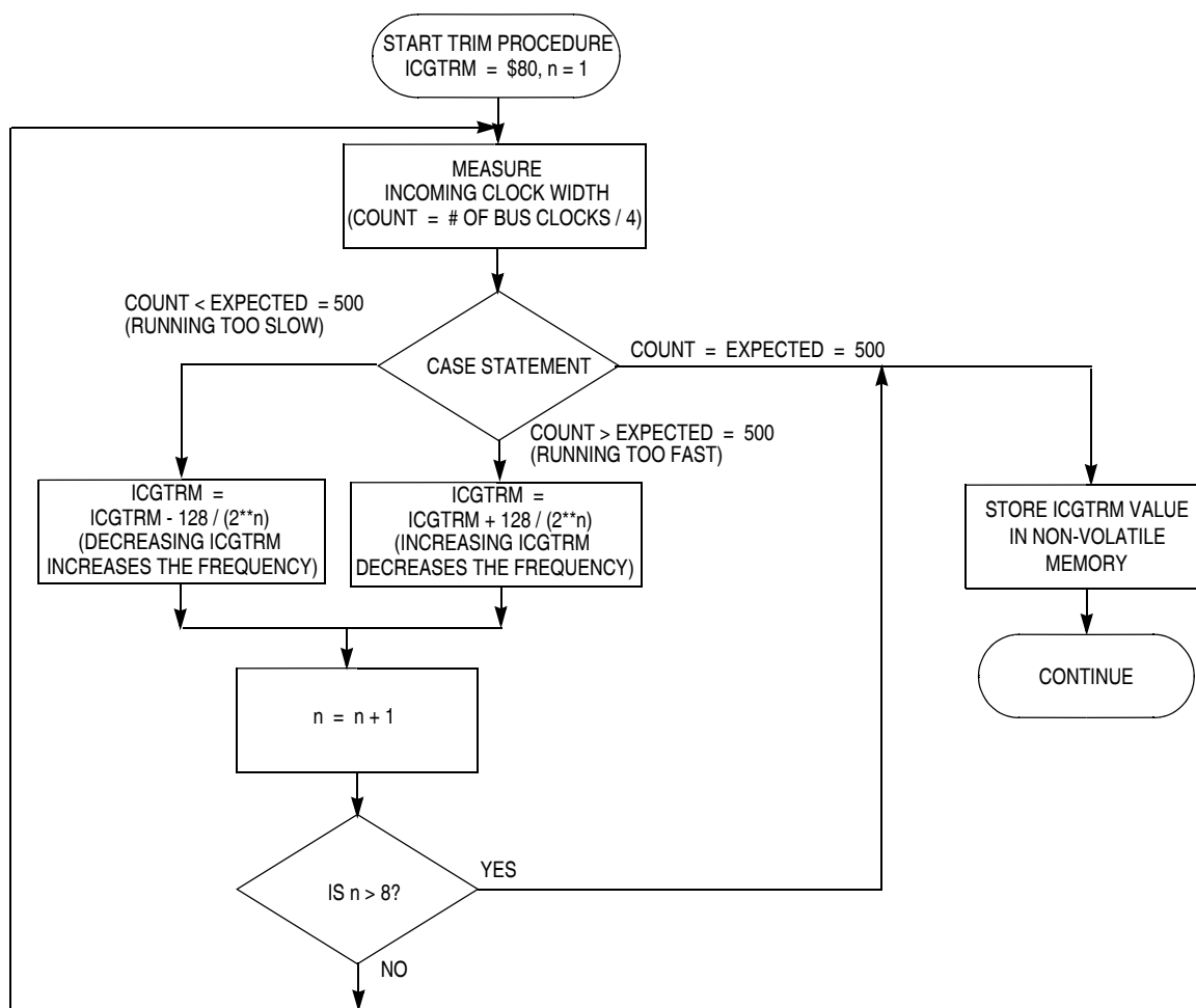
Figure 10-17. Trim Procedure
