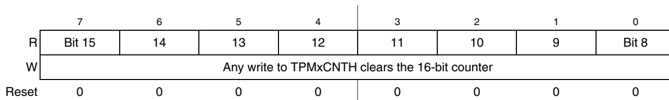
Figure 15-8. TPM Counter Register High (TPMxCNTH)
