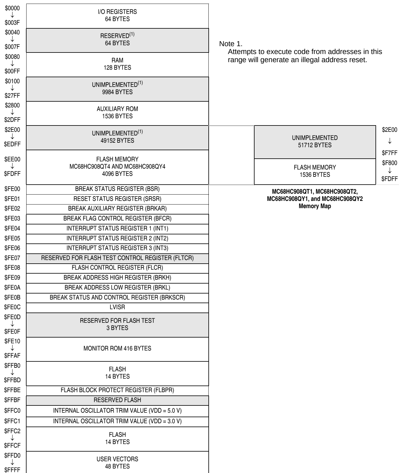
Figure 2-1. Memory Map
