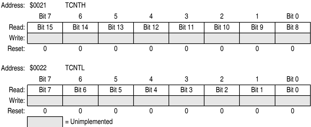
Figure 14-5. TIM Counter Registers (TCNTH:TCNTL)
