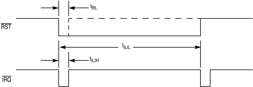
Figure 16-3. \overline{RST} and \overline{IRQ} Timing
