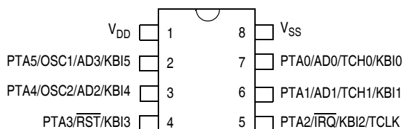
8-PIN ASSIGNMENT MC68HC908QT2 AND MC68HC908QT4 PDIP/SOIC
