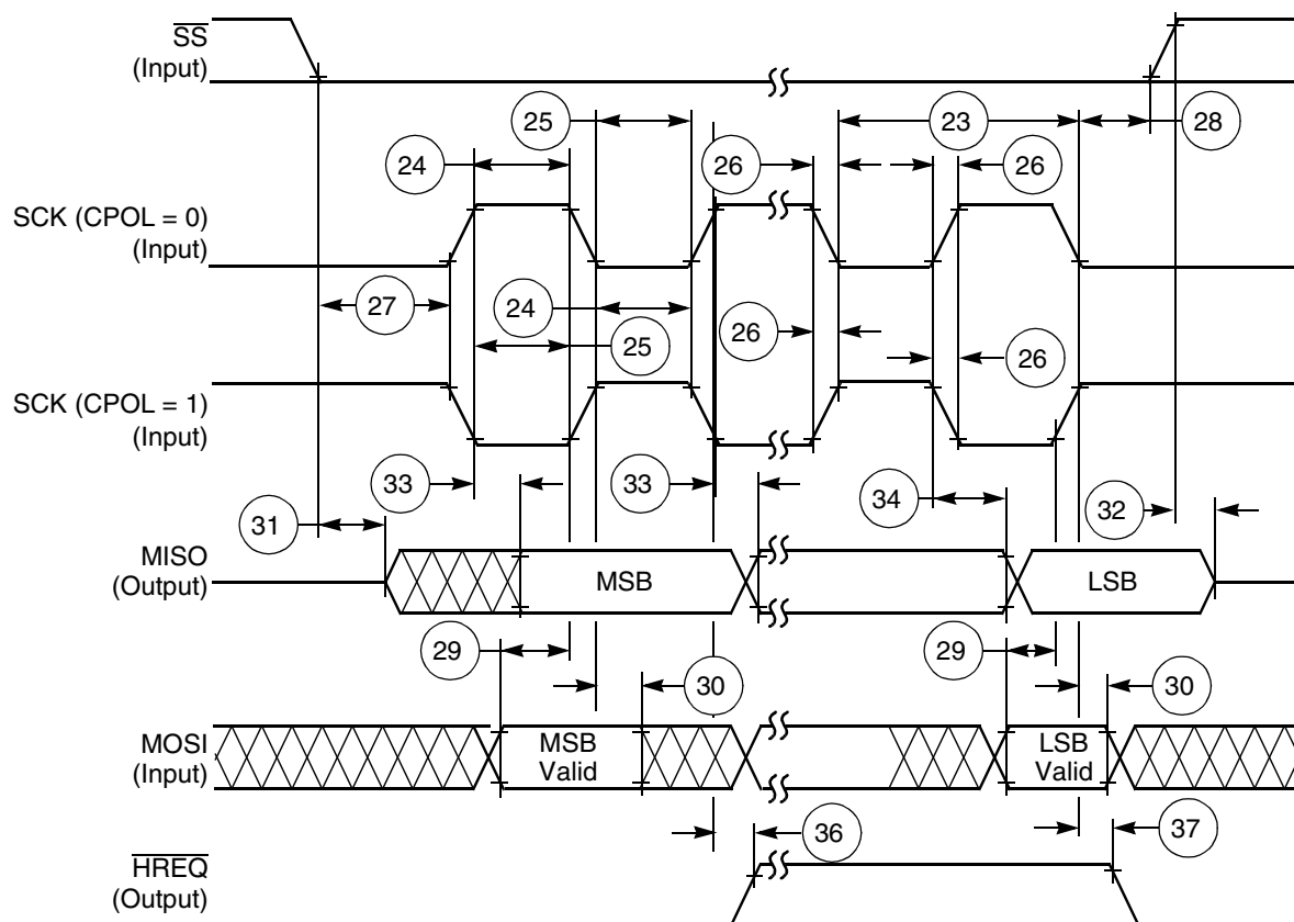
Figure 10. SPI Slave Timing (CPHA = 1)
